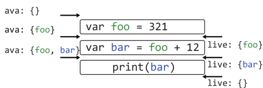
Fig. 2. Example of dynamic data flow analysis
