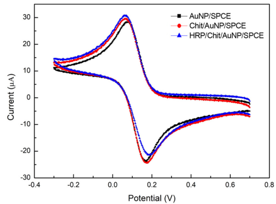
Fig. 3. Cyclic voltammograms of AuNP/SPCE, Chit/AuNP/SPCE and HRP/Chit/AuNP/SPCE.
