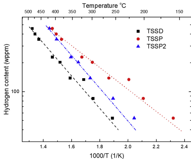
Fig. 2. Measured TSS of the hydrogen of Zirlo™
