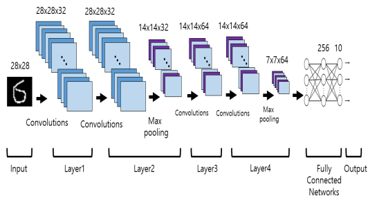
Fig. 5. Convolution neural network structure
