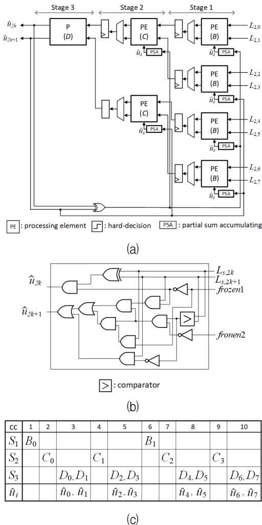
Fig. 6. 2-bit SC polar decoder (a) hardware architecture, P architecture, and (b) decoding scheduling when N = 8 [14].
