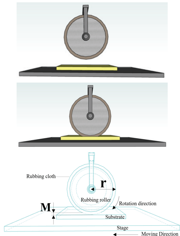
Fig. 2. Schematic diagram of rubbing machine.
