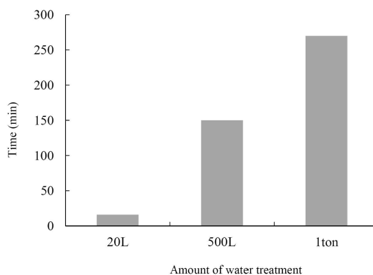
Fig. 2. Disinfection of bacteria according to seawater capacity by using plasma treatment.
