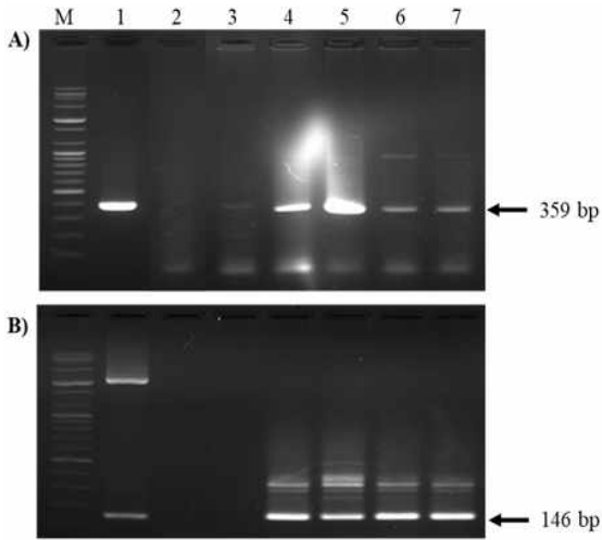
Fig. 1. Nested PCR assay for screening yellow head complex. A) First rounding PCR. B) Second rounding PCR. M: 100 bp DNA marker. Lane 1, positive control; Lane 2, negative control (without target DNA fragment). Lane 3-7; Shrimp samples.
