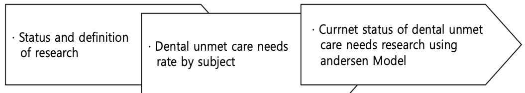
Fig. 1. Data extraction
