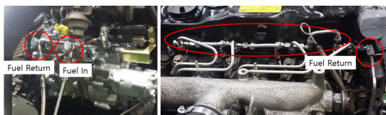
Fig. 2. Fuel system of test engine
