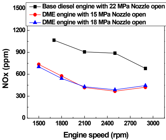
Fig. 7. The effect of nozzle open pressure on NOx emission
