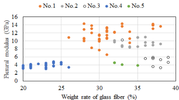
Fig. 3. Weight ratio of glass fiber vs. flexural modulus.
