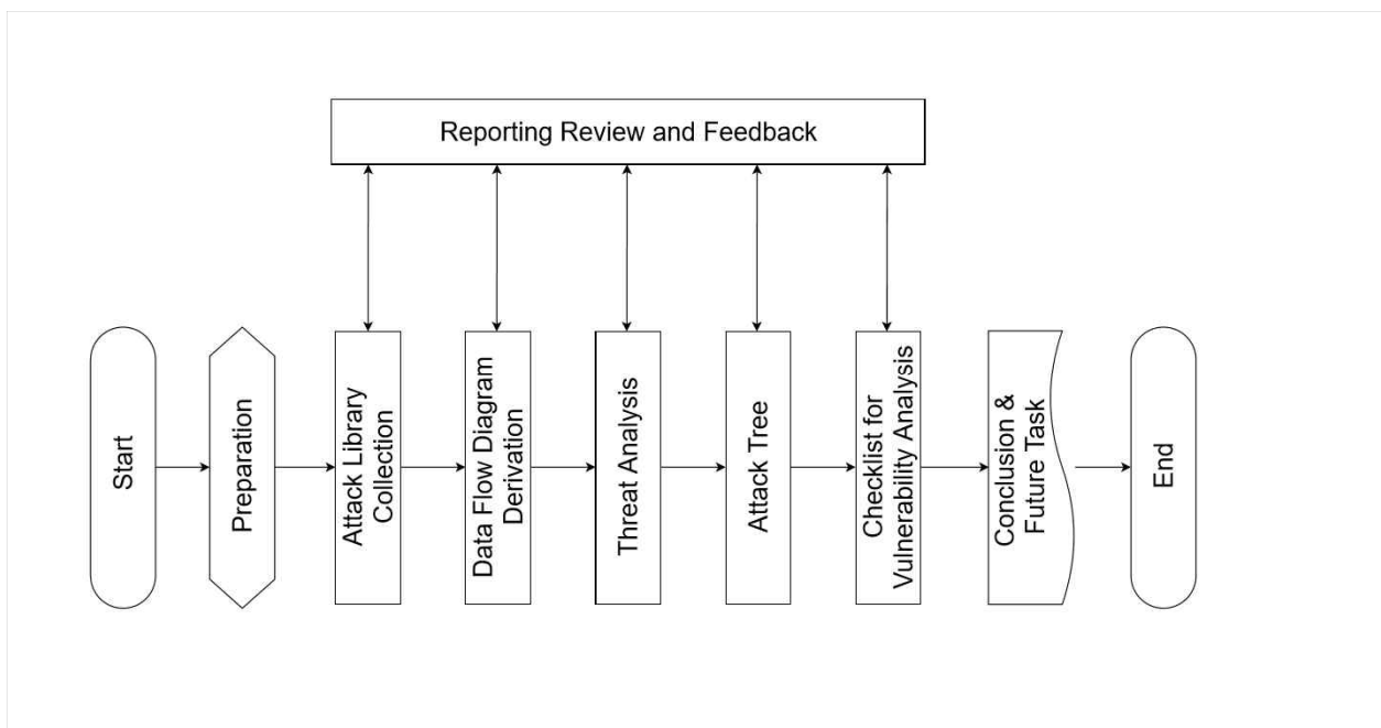
Fig. 1. Threat Modeling Procedure
