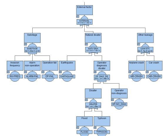
Fig. 2. Fault tree of external factor
