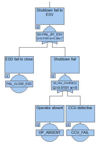
Fig. 8. Fault tree of ESV shutdown fail of internal factor
