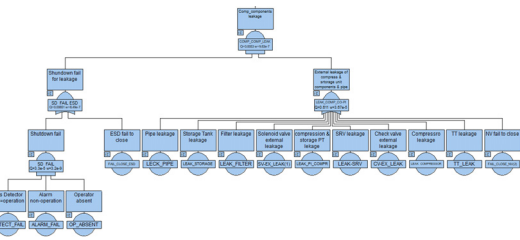
Fig. 4. Fault tree of compressor & storage unit component leak of Internal factor
