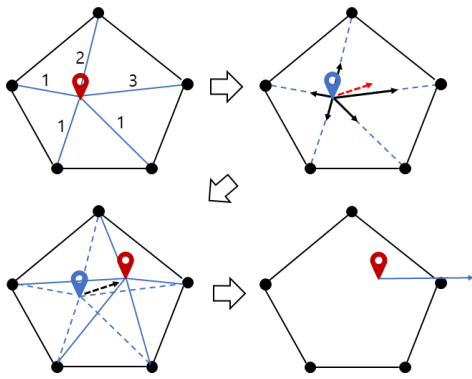
Fig. 5. Time-weighted Midpoint Search
