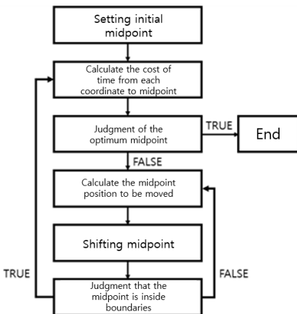
Fig. 3. Process for Obtaining Midpoint
