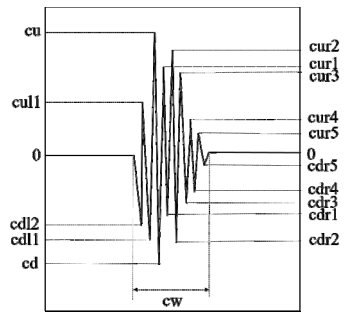
Fig. 2. Feature variables defined on a Chon pulse wave
