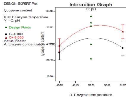
Fig. 4. Interaction graphs of enzyme concentration, reaction temperature and pH in lycopene extraction from autumn olive berry
