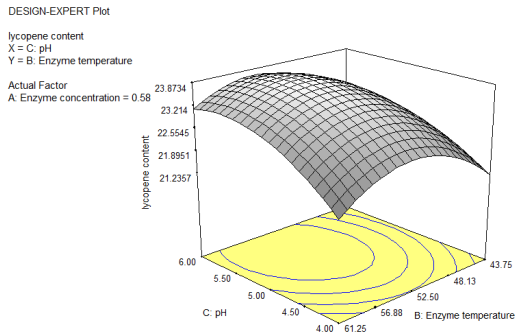
Fig. 3. Interaction graphs of enzyme concentration, reaction temperature and pH in lycopene extraction from autumn olive berry
