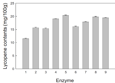
Fig. 2. Lycopene extraction yields from autumn olive berry using various enzymes. (1) Control; (2) Celluclast; (3) AMG; (4) Promozyme; (5) Ceremix; (6) Viscozyme; (7) Ultraflo; (8) Pectinex; (9) Tunicase.
