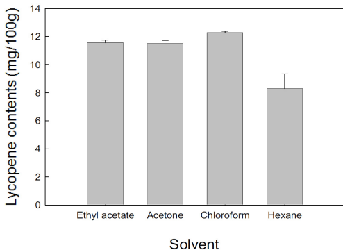
Fig. 1. The lycopene extraction yields from autumn olive berry by the treatment with different solvents
