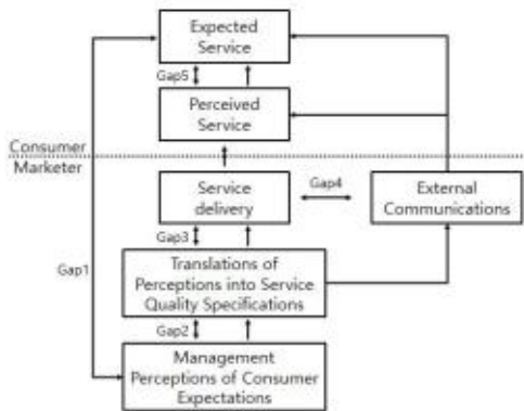
Fig. 2. Gap Model
