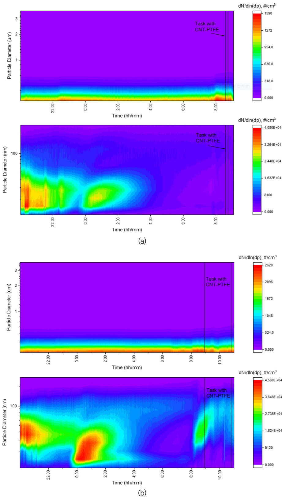
Figure 1. Particle size distributions measured by SMPSs and OPSs; (a) powder supply, and (b) CNC machining
