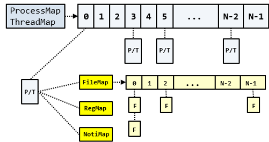
Fig. 5. Monitoring data structure
