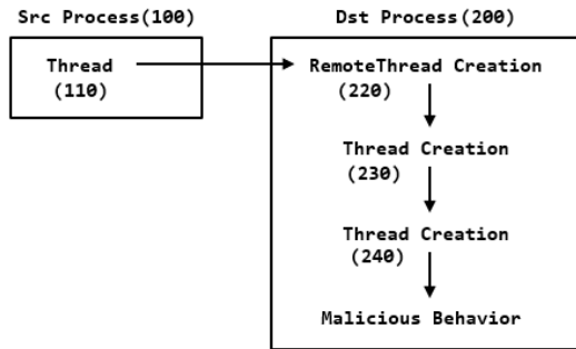
Fig. 3. Malicious behavior case caused by the RemoteThread's derived thread
