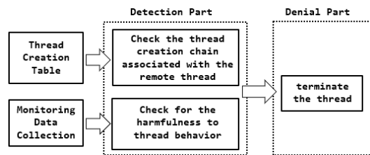
Fig. 6. Overview of thread behavior based detection and denial
