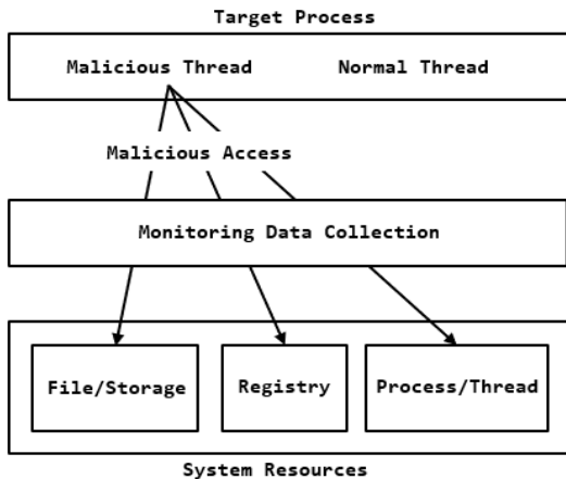
Fig. 4. Thread based monitoring
