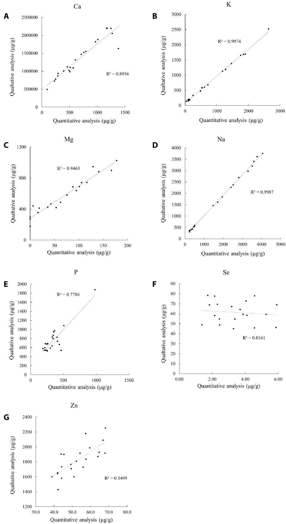
Fig. 1. Correlation of quantitative and qualitative analysis in ICP. The correlation between quantitative and qualitative data of (A) calcium, (B) potassium, (C) magnesium, (D) sodium, (E) phosphorus, (F) selenium, (G) zinc. ICP, inductively coupled plasma.
