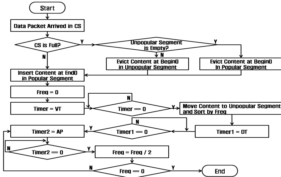
Fig. 2. DA-LFU Flowchart of Algorithms
