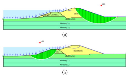
Fig. 5. Pre-earthquake stability of levee (a) Landside (b) Waterside
