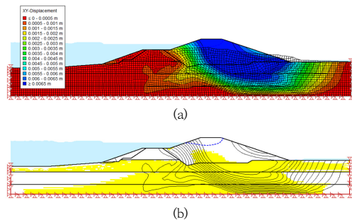
Fig. 9. Deformation of the levee after the earthquake (a) Displacement (b) Yield area
