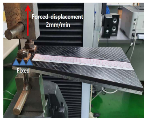
(b) Out-plane load(Mode III)
