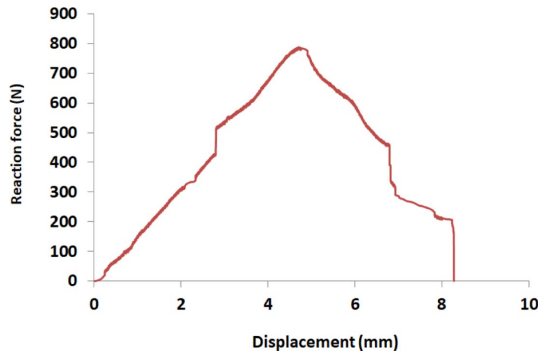
Fig. 7. Reaction force due to forced displacement (CFRP-Al6061) (Mode III)
