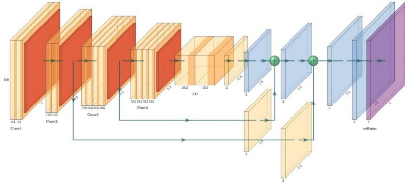
Fig. 4. Model architecture. Both modified models have reduced number of parameters
