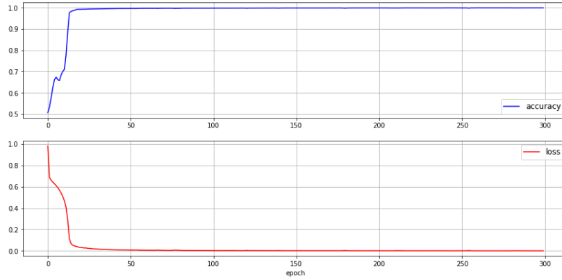
Fig. 6. Model, training accuracy, and loss for Type 2. At epoch 300, training loss approached 0.001
