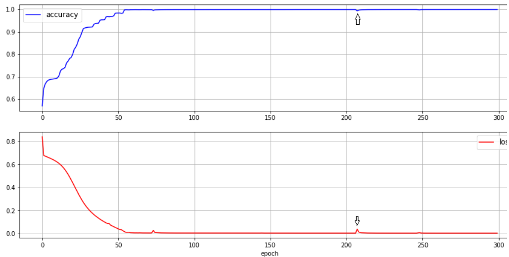
Fig. 5. Model, training accuracy and loss at each epoch for Type 1. At epoch 300, training loss approached 0.001
