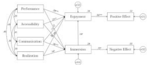
Fig. 1. Hypothetical Path Model
