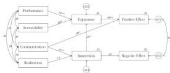
Fig. 2. Modified Path Model
