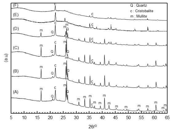
Fig. 5. XRD patterns of coal tailing with the different added amount of \text{Na}_2\text{CO}_3 at 1,450 °C; the added amount of \text{Na}_2\text{CO}_3 : (A) 0.5 wt.%, (B) 1 wt.%, (C) 2 wt.%, (D) 5 wt.%, (E) 10 wt.%, and (F) 20 wt.%.
