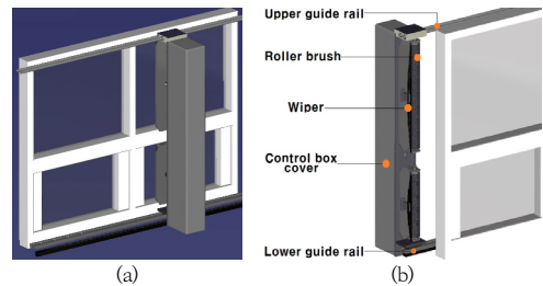
Fig. 3. A concept of a guide rail fixed cleaning device (a) Outer view (b) Inner view
