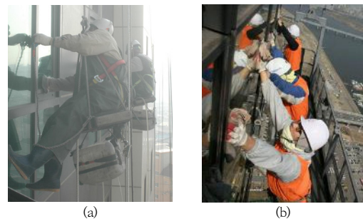
Fig. 1. Windows cleaning method by workers (a) Wet process using scaffolds[2] (b) Dry process using a gondola[3]
