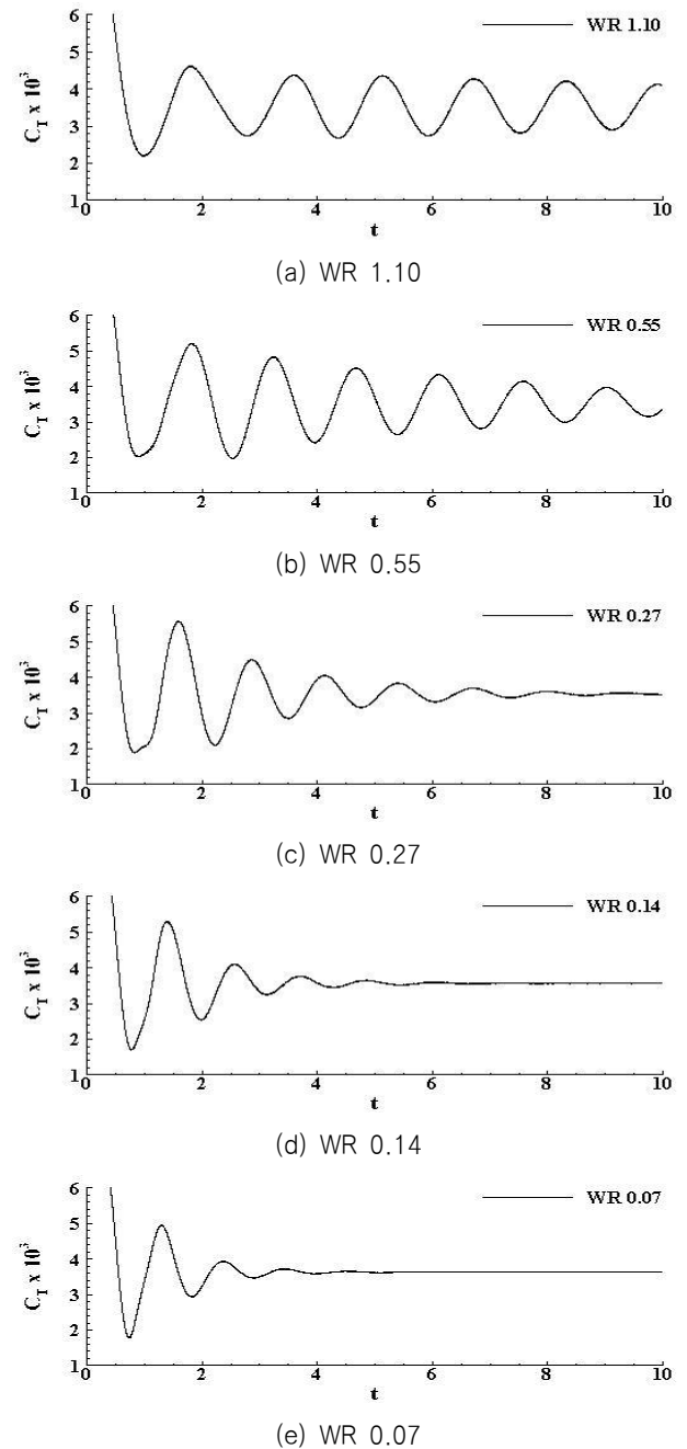
Fig. 6 Time histories of total resistance coefficients for various WR
