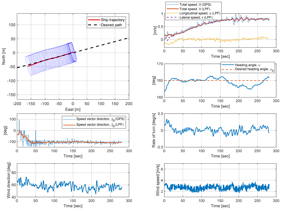
Fig. 6 Crabbing test results (case 3)
