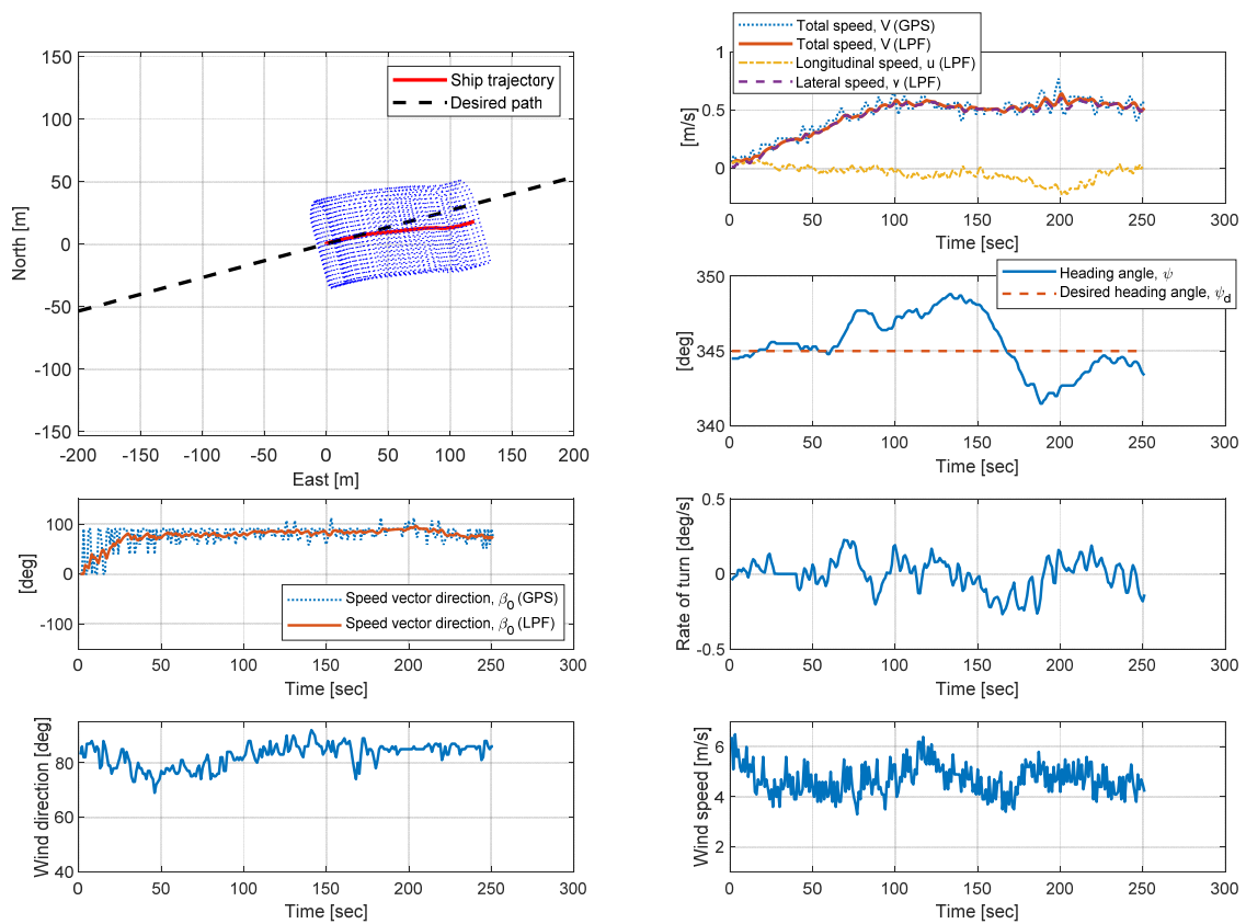
Fig. 5 Crabbing test results (case 2)
