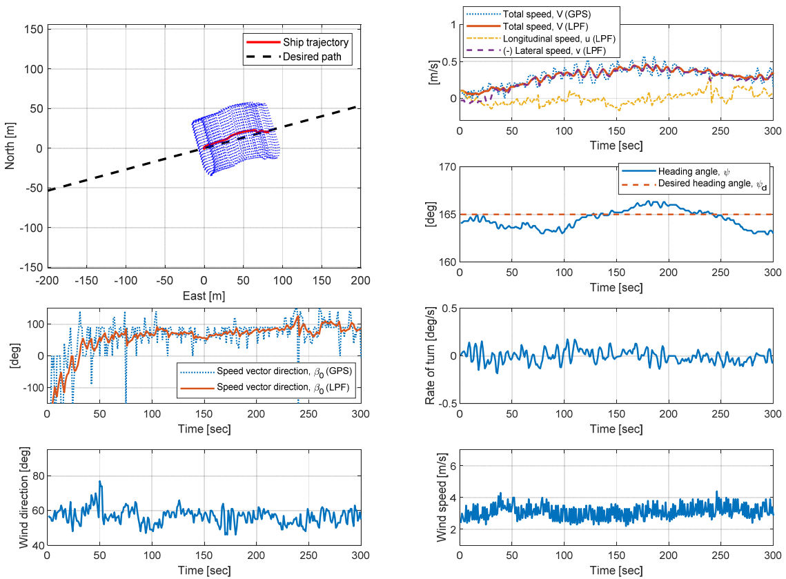
Fig. 7 Crabbing test results (case 4)
