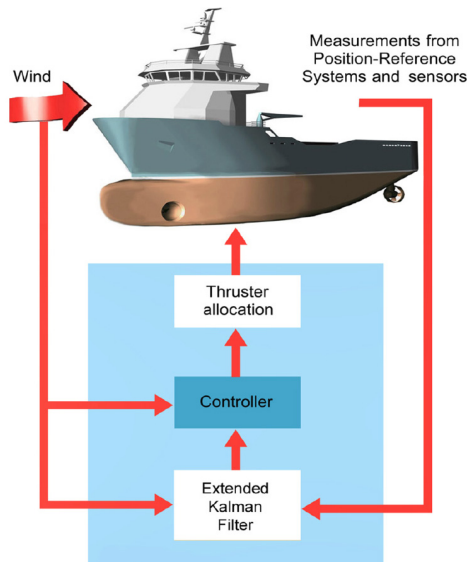
Fig. 2 K-POS dynamic positioning system block diagram (Lee et al., 2018)
