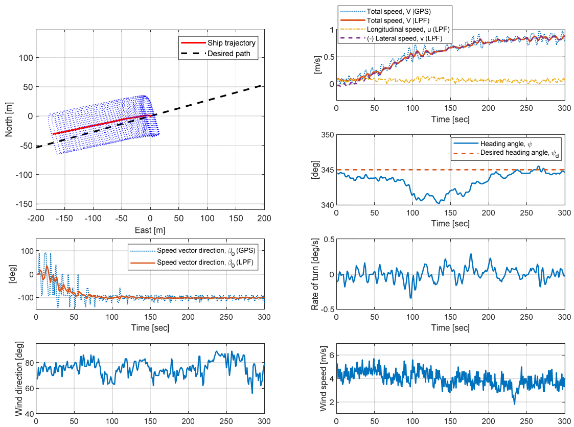
Fig. 4 Crabbing test results (case 1)
