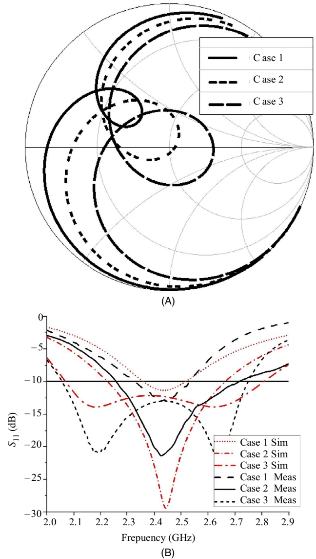
FIGURE 5 Effects of change in Z_{11} for different values of C_f and L_r . (A) Curves of Z_{in} on smith chart. (B) Effect on return loss
