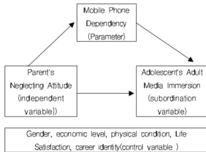
Fig. 1. Research model
