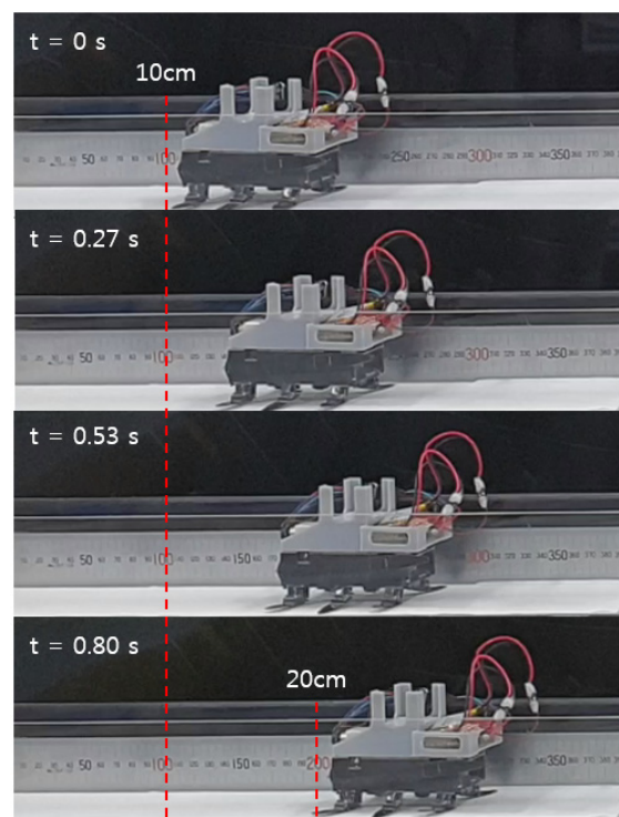
[Fig. 12] Running of the six-leg crawling robot. Captured in the measurement video
