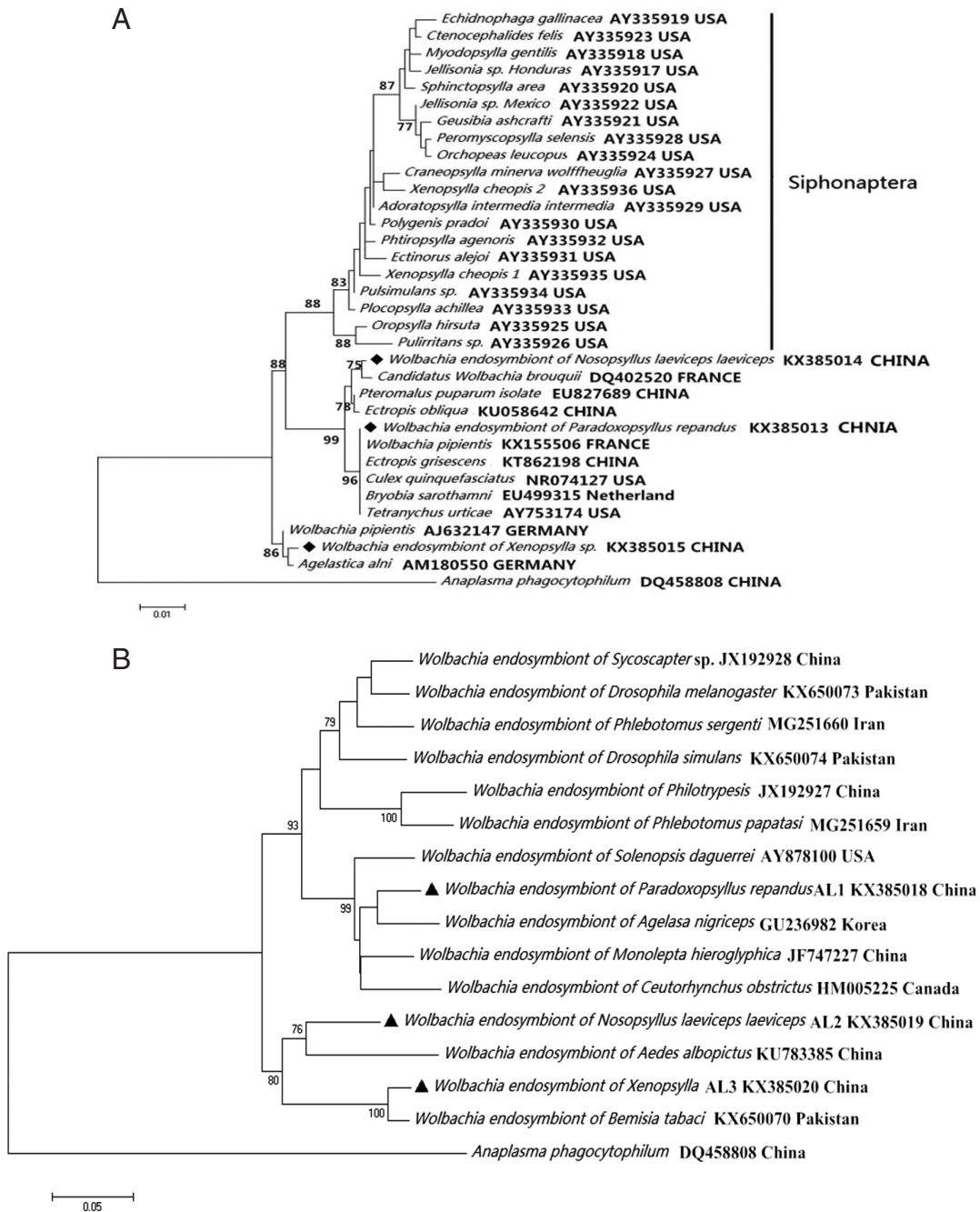
Fig. 2. Wolbachia (◆, ▲) collected from Nosopsyllus laeviceps laeviceps , Xenopsylla sp., Paradoxopsyllus repandus . Phylogenetic trees of (A) 16S rRNA and (B) wsp sequences. Maximum-likelihood (1,000 bootstrap replicates) and neighbour-joining (500 bootstrap replicates) were applied.
