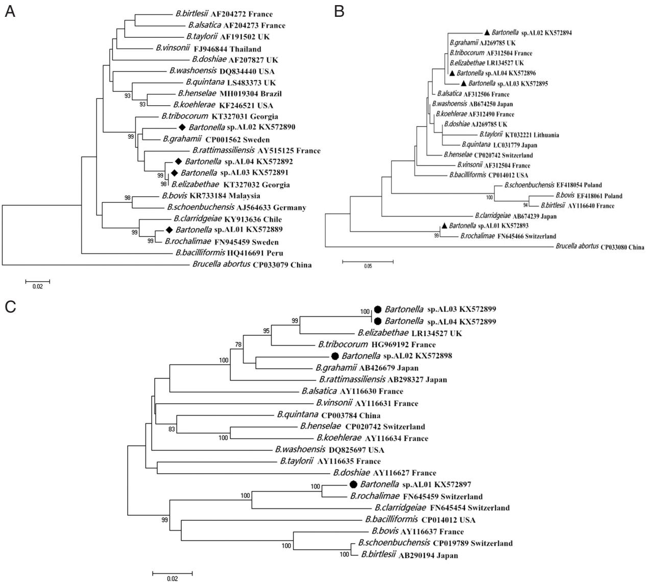
Fig. 1. Maximum likelihood (ML; 1,000 bootstrap replicates) and neighbor joining (NJ; 500 bootstrap replicates) phylogenetic tree of the (A) gltA , (B) ITS , and (C) ribC genes. Bartonella sp. sequences AL01-04 (◆, ▲, ●) obtained in this study.
