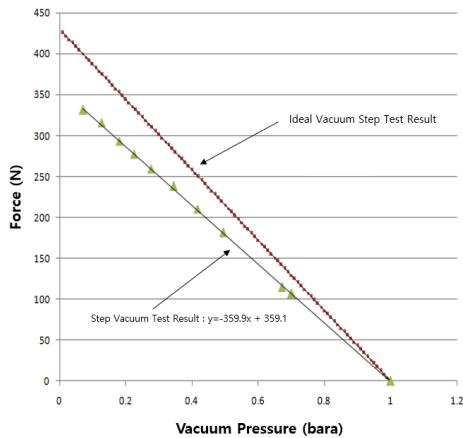
Fig. 5. Result of Vacuum Step Test
