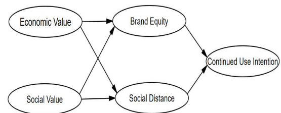
Fig. 1. Research model
