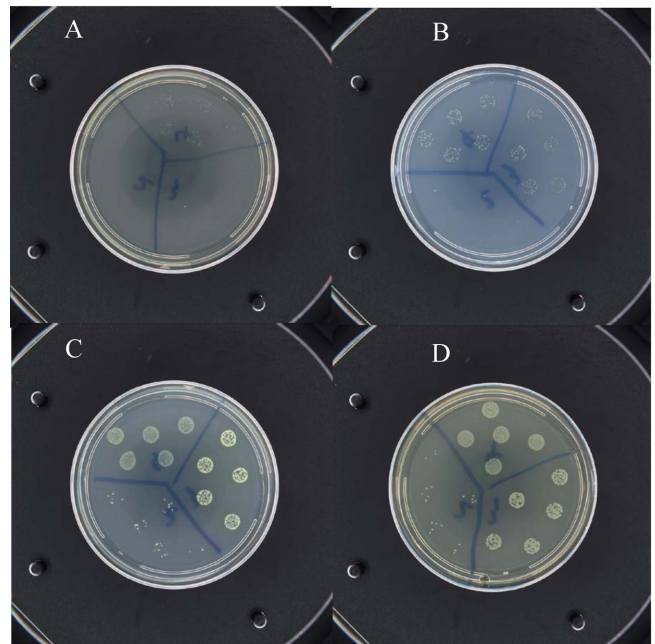
Fig. 2. Plate images of B. cenocepacia AU19236 grown on TSA (A), 1/10 × TSA (B), 1/3 × R2A (C), and R2A (D) media stored at 42°C for 42 days.
