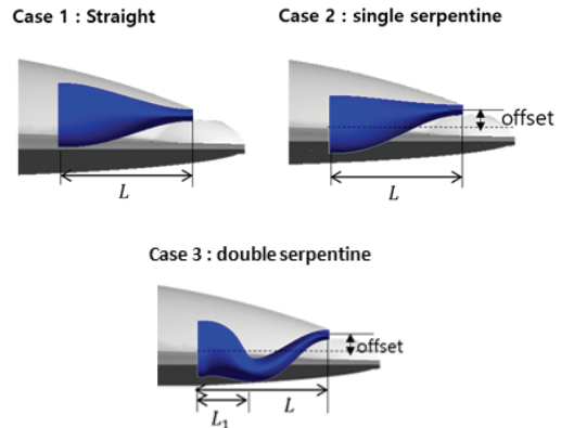
Fig. 3 Shape of straight, single and double serpentine nozzle.
