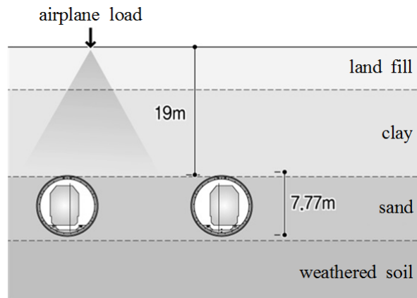
Fig. 6. Ground condition
