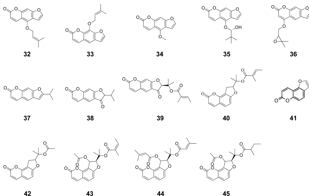
Fig. 4. Chemical structure of the psoralen-type coumarins in A. decursiva .
