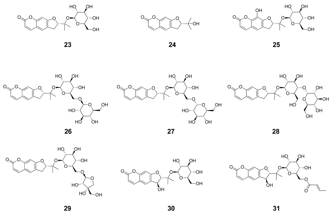
Fig. 3. Chemical structure of the dihydropsoresalen-type coumarins in A. decursiva .
