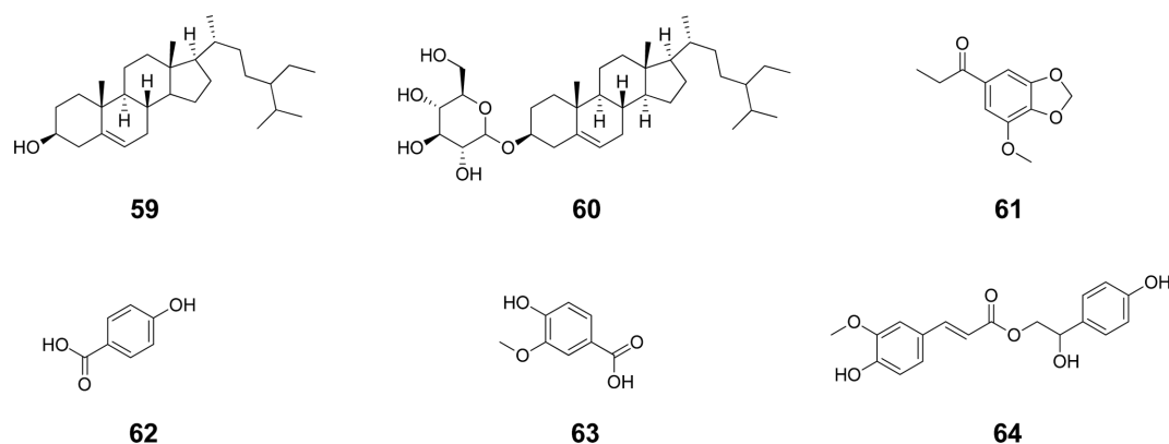
Fig. 7. Chemical structure of the other constituent in A. decursiva .
