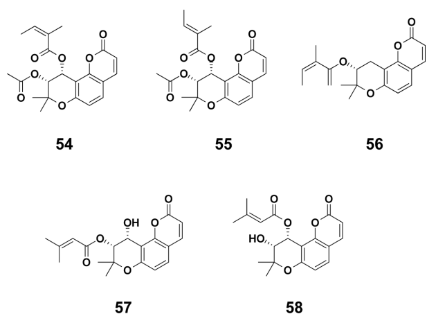
Fig. 6. Chemical structure of the dihydropyran-type coumarins in A. decursiva .
