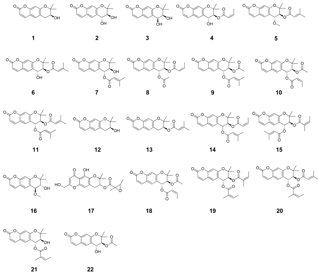
Fig. 2. Chemical structure of the major dihydroxanthyletin-type coumarins in A. decursiva .
