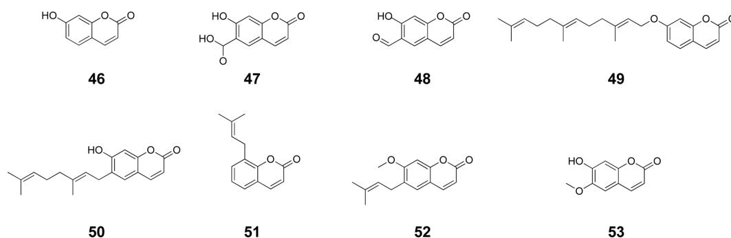
Fig. 5. Chemical structure of the hydroxycoumarins in A. decursiva .
