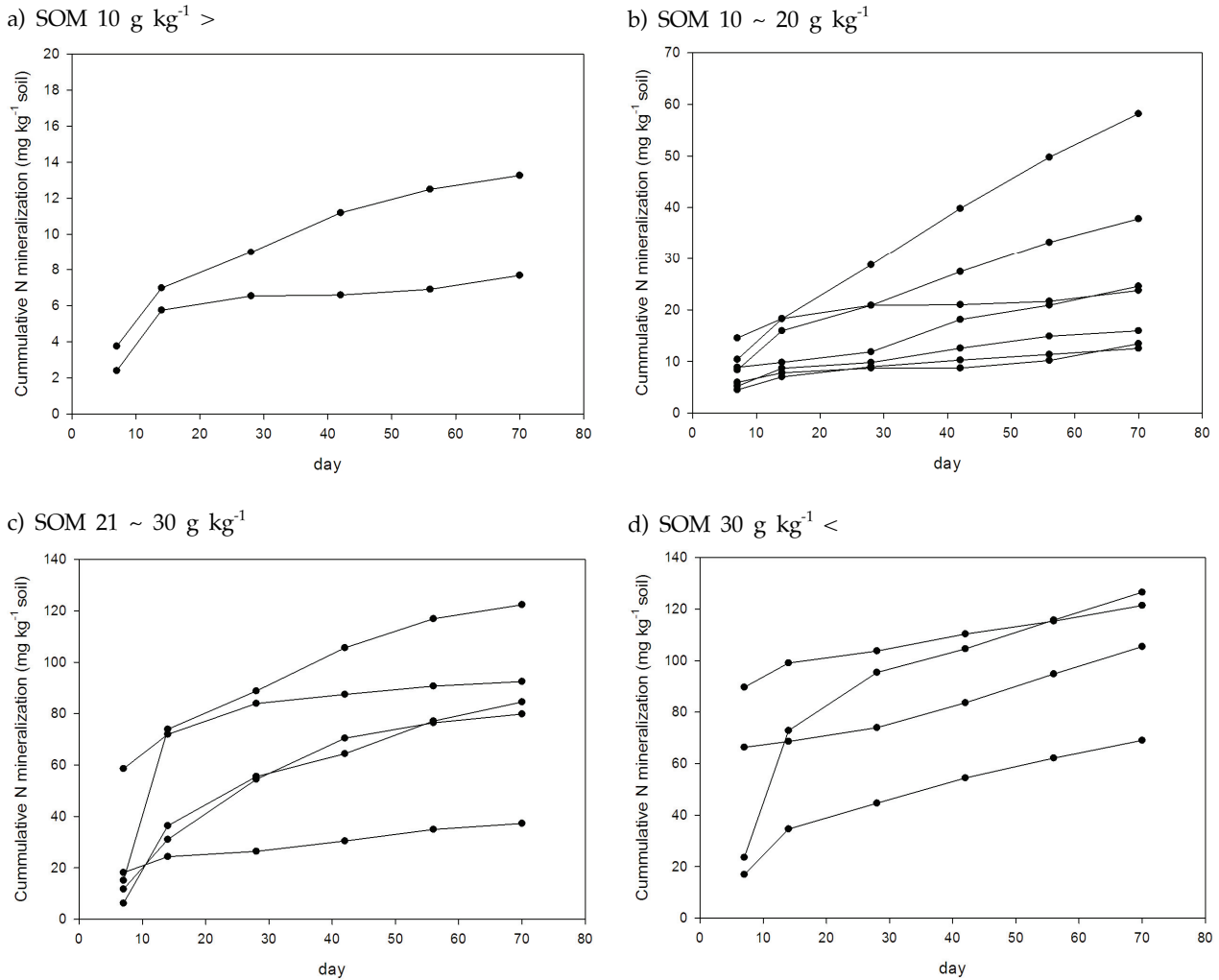
Fig. 2. Cumulative N mineralization at 30°C for 70 days according to soil organic matter range, under 10 g kg -1 (n=2), 10~20 g kg -1 (n=7), 21~30 g kg -1 (n=5) and above 31 g kg -1 (n=4).
