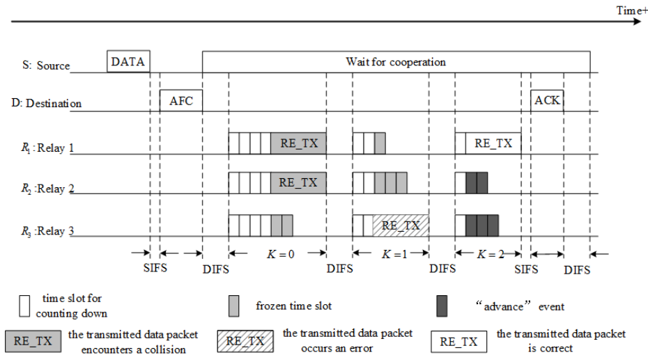
Fig. 4. An operational example of SPRCSMA
