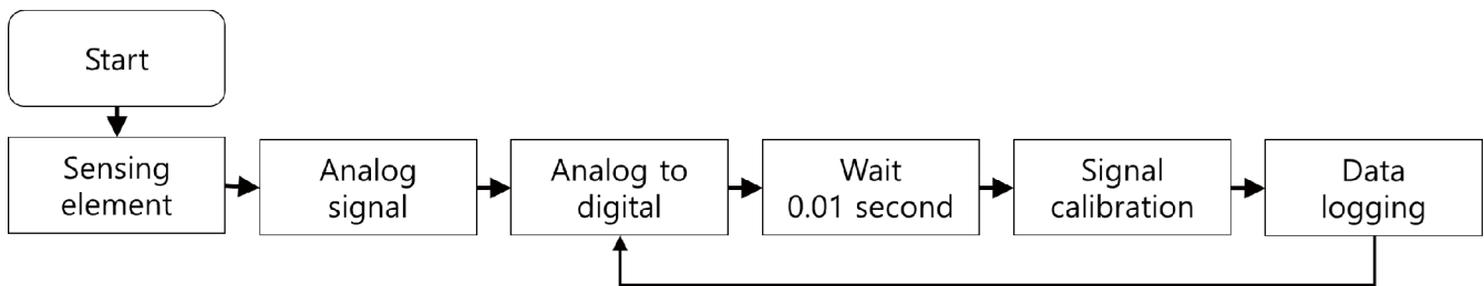
Fig. 2. Flow chart of signal processing to log the distance between the sensors and sow's side surface in 100 Hz of measurement of frequency.
