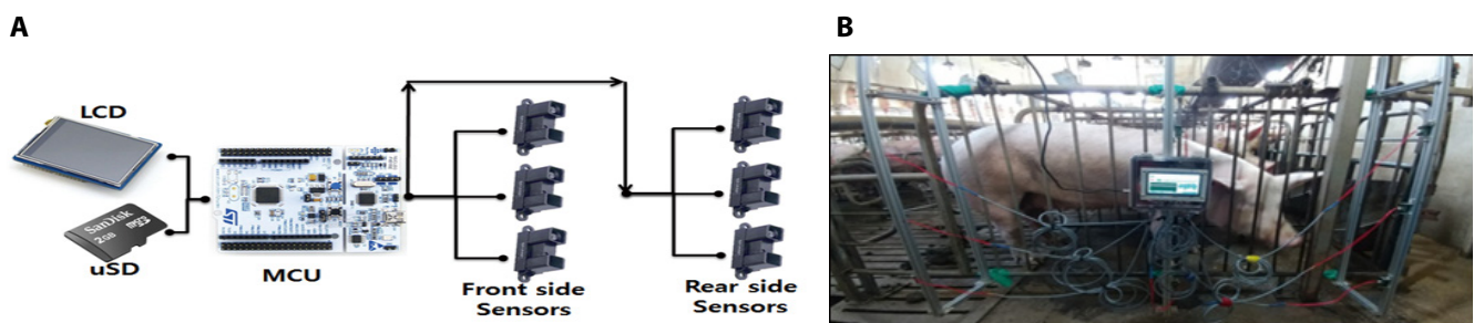
Fig. 1. (A) Standing sensor connecting diagram image. (B) Installed standing sensor image.
