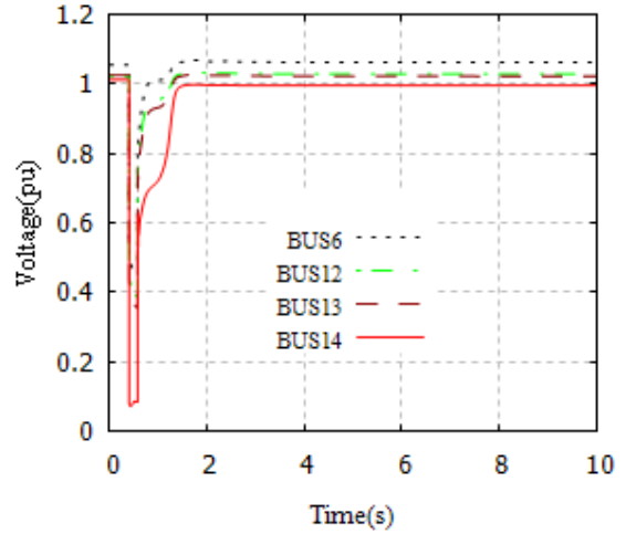
Fig. 8. Voltage Response with Wind-Turbine Generator at the BUS8 and ESS 60% Active Power Supply at the BUS14
