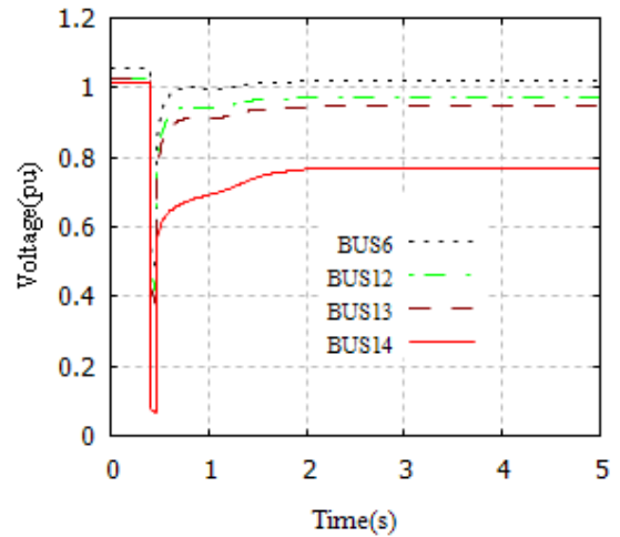
Fig. 2. Voltage Response with Wind-Turbine Generator at the BUS2
