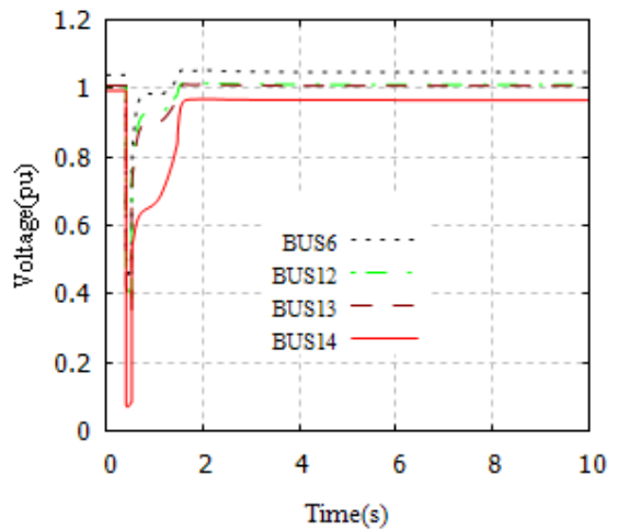
Fig. 6. Voltage Response with Wind-Turbine Generator at the BUS3 and ESS 100% Active Power Supply at the BUS14
