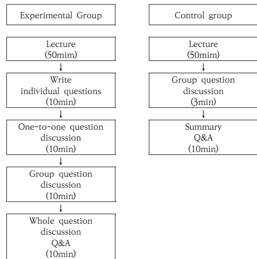
Fig. 1. Program process
