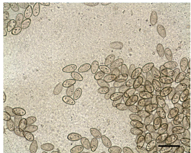
Fig. 2. Numerous C. sinensis eggs in a smear of bile juice drained from the leopard cat. Various characteristics like small operculum, shouldering and developed miracidium were partially observed in some of the eggs. Bar=50 \mu\text{m} .
