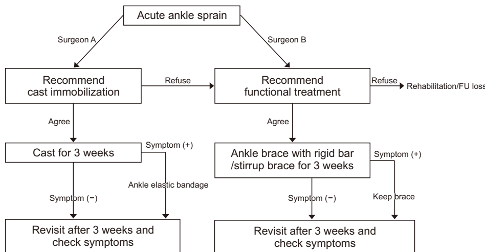
Figure 1. Treatment algorithm.
