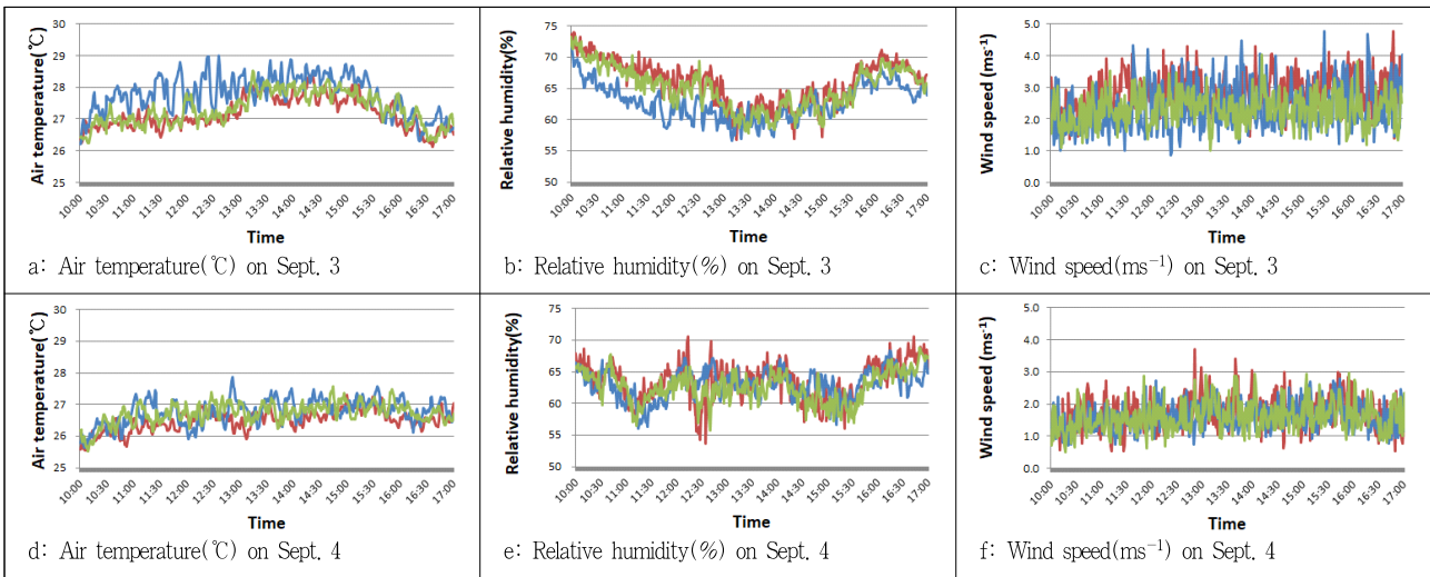
Figure 3. The measured microclimatic data Legend: — Natural grass — Artificial grass — Clay sand
