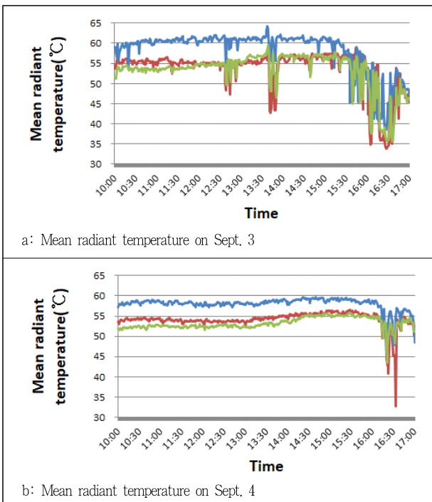
Figure 7. Mean radiant temperature results Legend: — Natural grass — Artificial grass — Clay sand
