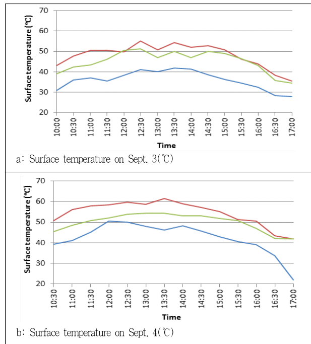
Figure 4. The measured surface temperature Legend: — Natural grass — Artificial grass — Clay sand
