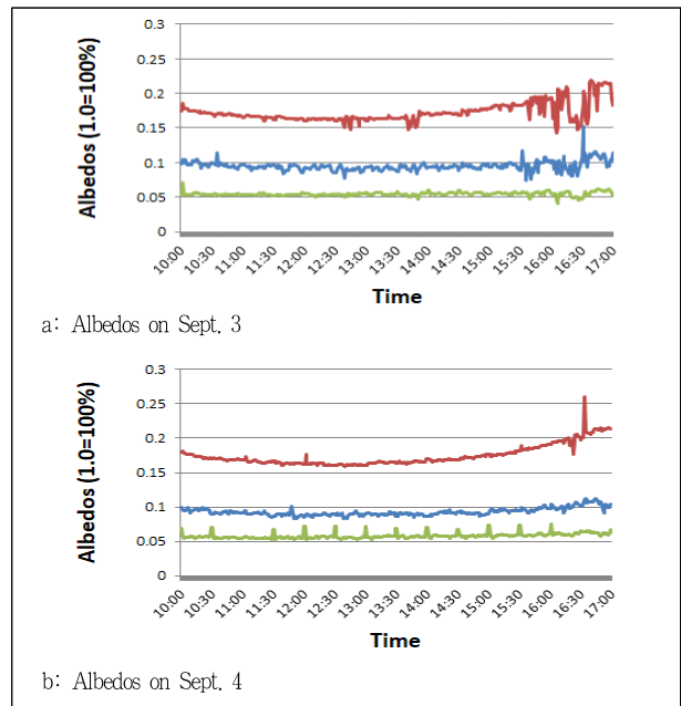
Figure 6. The measured albedos(1.0=100%) Legend: — Natural grass — Artificial grass — Clay sand
