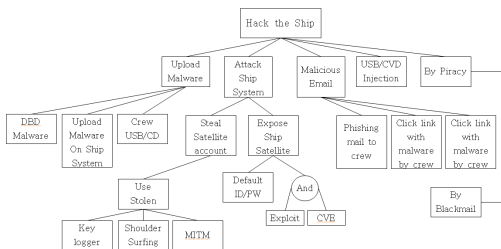
Fig. 3. Attack tree
