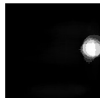
Fig. 11. PSR Image
