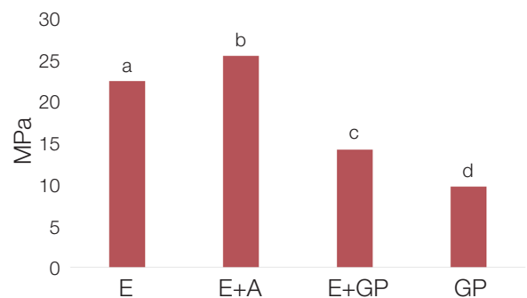
Fig. 2. Scheffe's test result of shear bond strength of LightFix. The different alphabet characters on the bars indicate the significant difference ( P < 0.05 ). E: Etching; E+A: Etching+Adhesive resin; E+GP: Etching+G-Premio Bond; GP: G-premio Bond.
